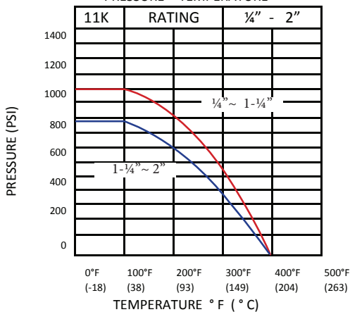
PRESSURE - TEMPERATURE
