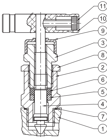
SECTIONAL DETAILS OF VALVE
